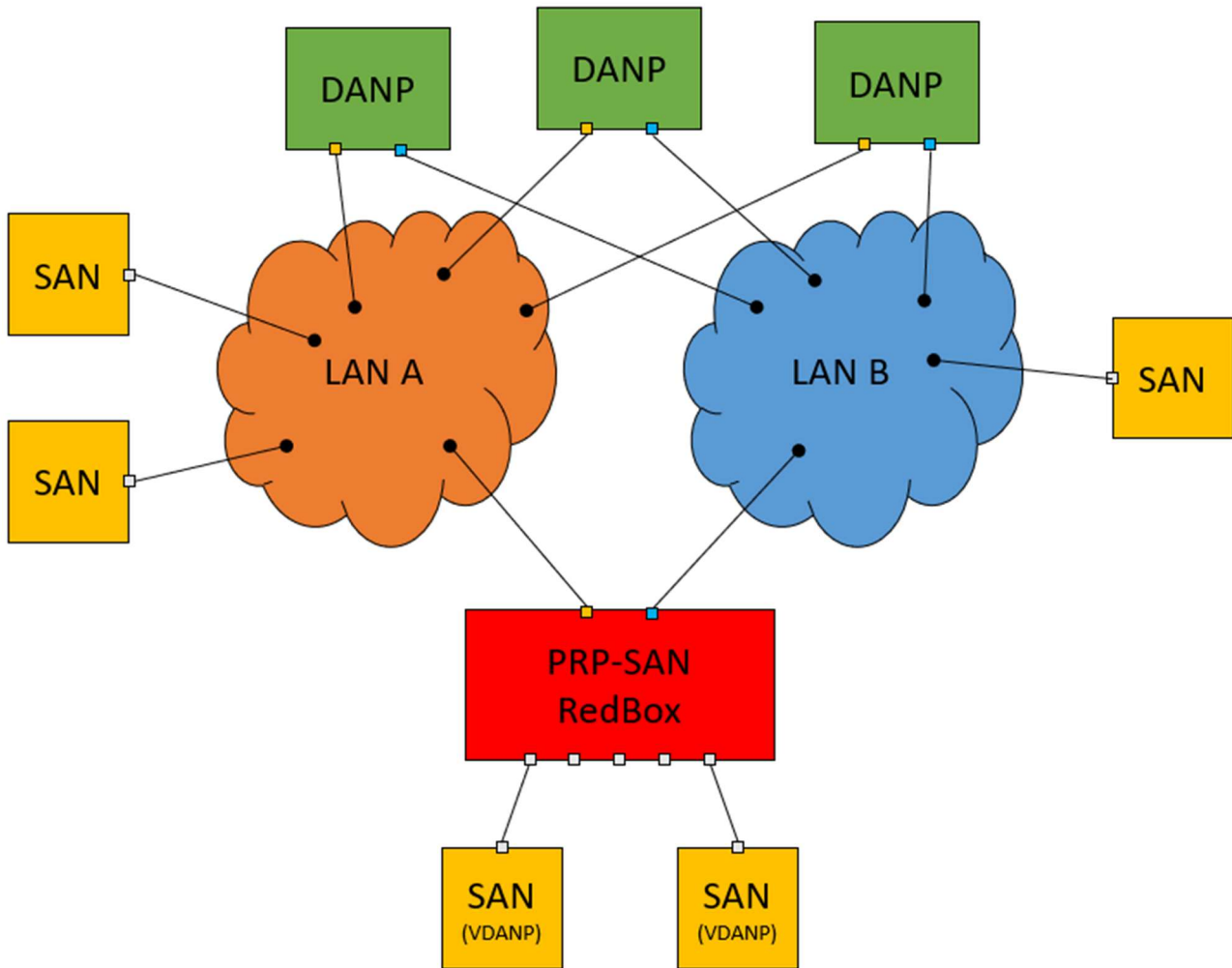
Figure 2.134 A PRP-SAN RedBox connected to a PRP network
