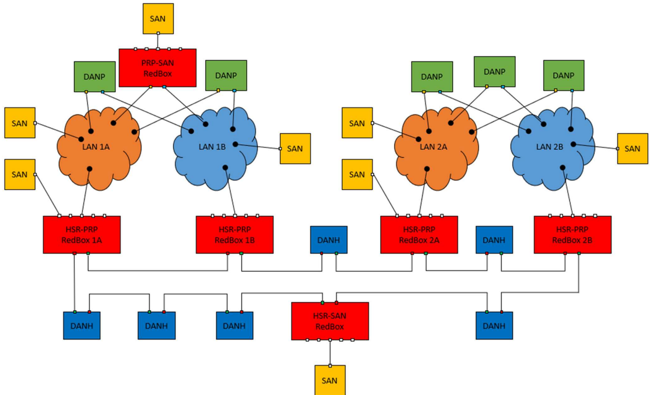
Figure 2.137 Multiple PRP networks connected to a single HSR ring
