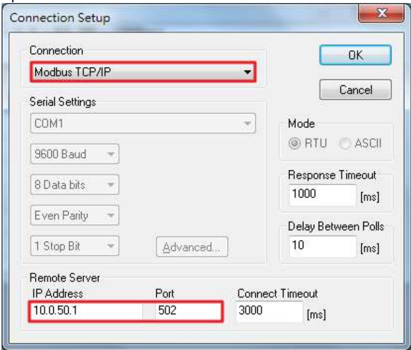
Figure 2.122 Modbus Poll Connection Setup
