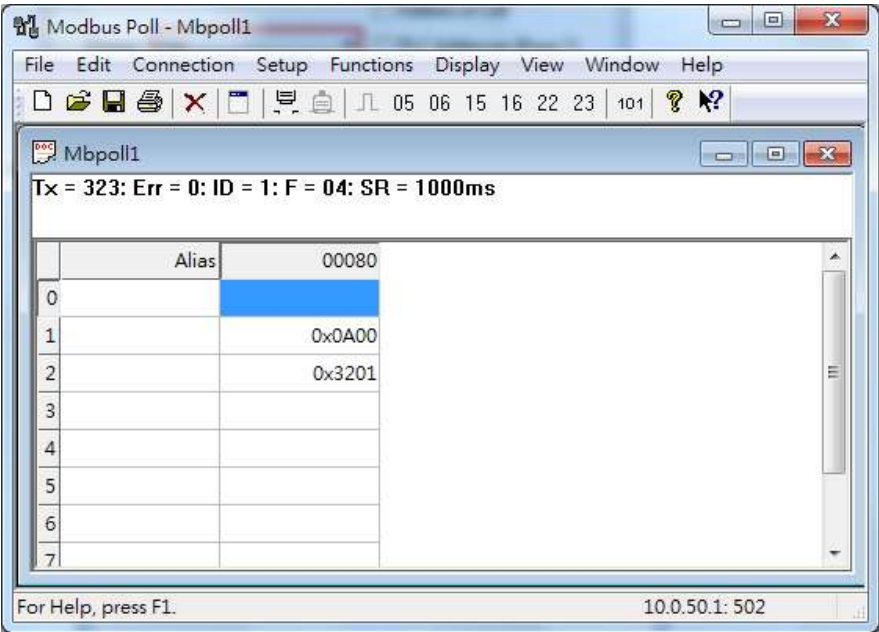
Figure 2.132 Modbus Memory Address 81 and 82 are the location of RHG9728’s IP Address
