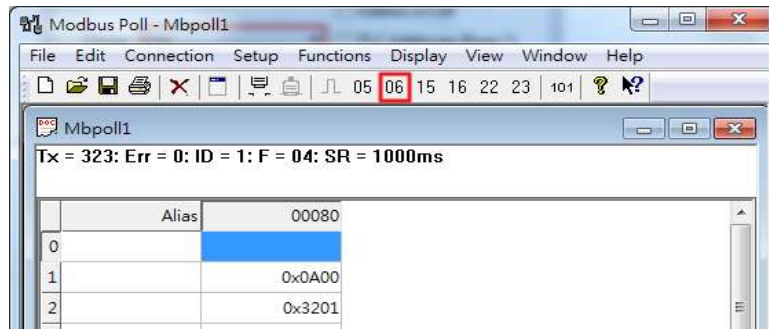
Figure 2.131 Click on Function 06 in the Modbus Poll
