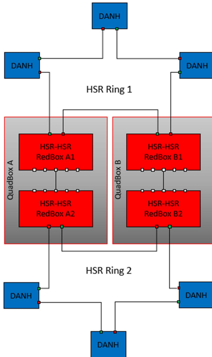
Figure 2.139 Connection of two HSR rings with two QuadBoxes
