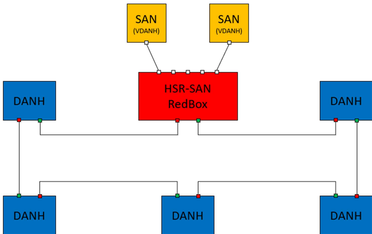
Figure 2.135 An HSR-SAN Redbox connected to an HSR ring
