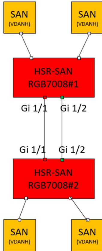
Figure 2.140 Demonstration of HSR-SAN
