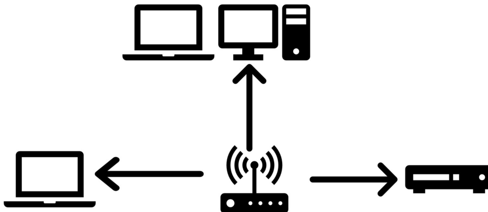
Figure 2.109 Traffic Mirroring Operation
