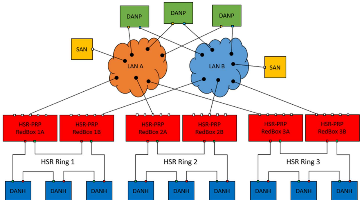
Figure 2.138 Single PRP network connected to multiple HSR rings
