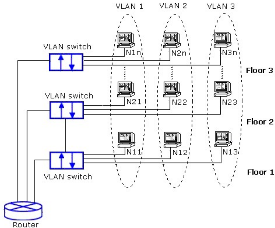
Figure 2.86 Example of VLAN Configuration
