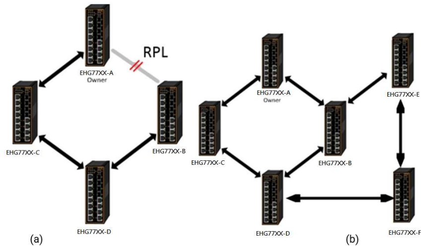
Figure 2.28 An Example of Ring Topology (a) Major Ring, and (b) Sub-Ring
